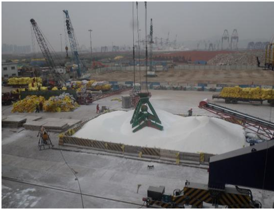
The fertilizer is being loaded on board by grab
