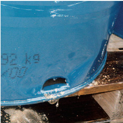
Drums stabbed by forklift – a common cause of drum damage during handling
